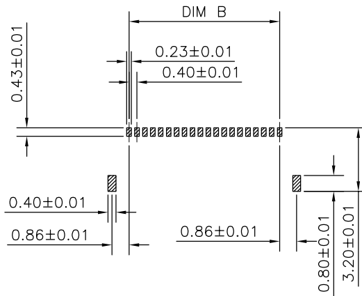
RECOMMENDED METAL MASK PATTERN METAL MASK THICKNESS: WHEN 120 μm (TERMINAL PORTION OPENING AREA RATIO:86%)
